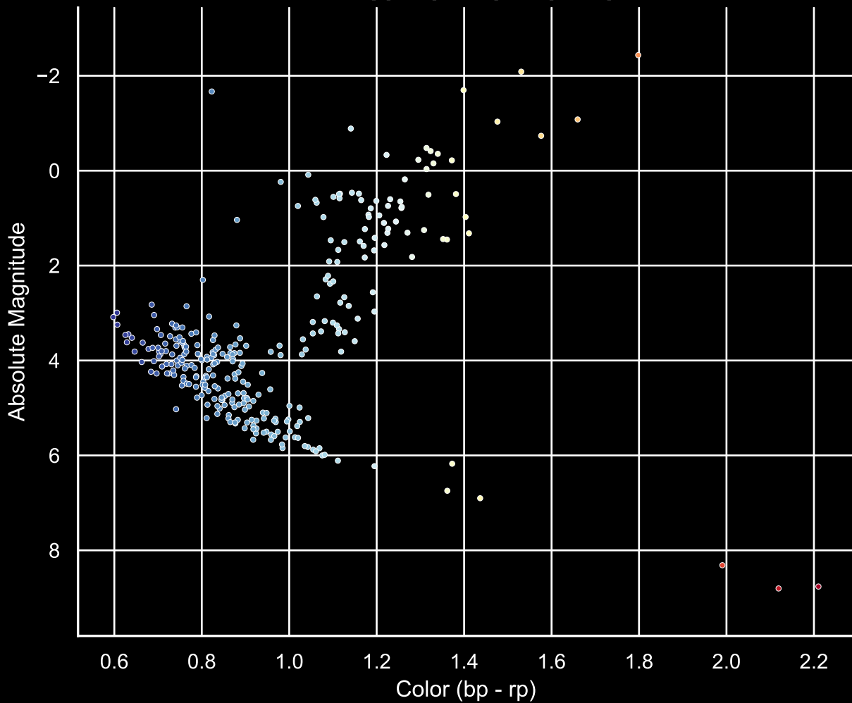
GALAH Hertzprung-Russel Diagram Field [3] Ra [331.14] Dec [-55.76]
