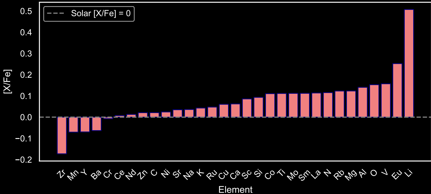
Abundance Pattern for GALAH Star Field [3] (N=308)
