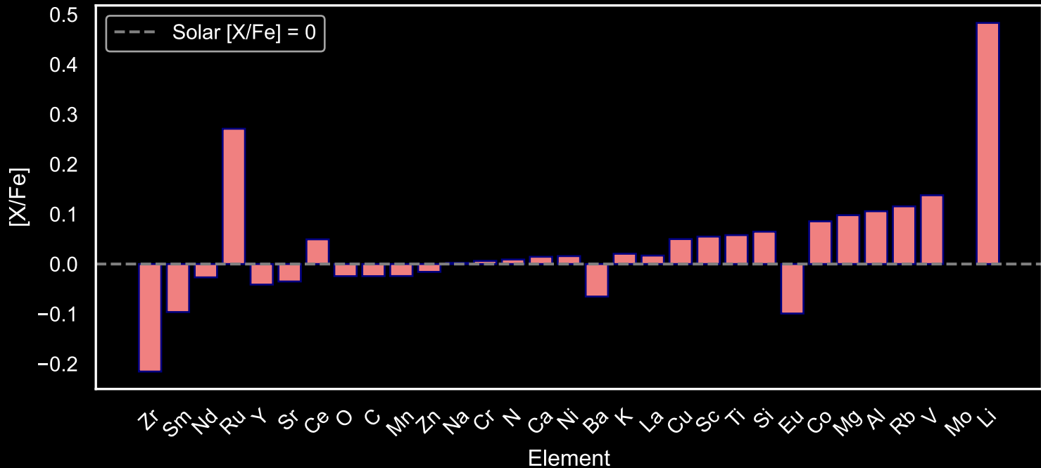
Abundance Pattern for GALAH Main Sequence Stars: Star Field [3] (N=134)
