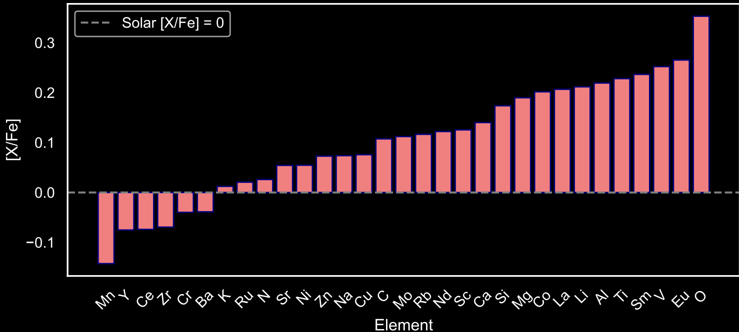
Abundance Pattern for GALAH Red Giants: Star Field [3] (N=81)
