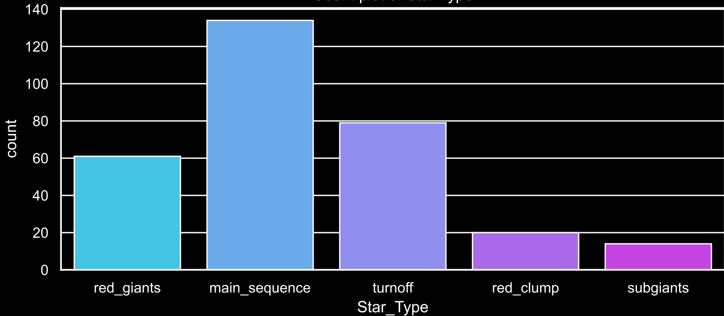
Field [3] Count plot of Star Type
